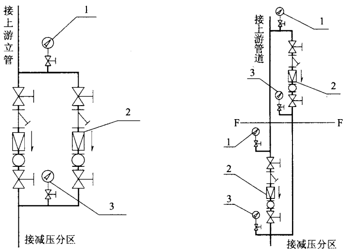
(a) 减压阀并联阀组同层布置
